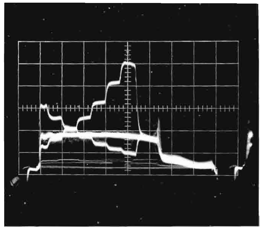
FIG. 10A M channel with white chip exposed just below the knee.
