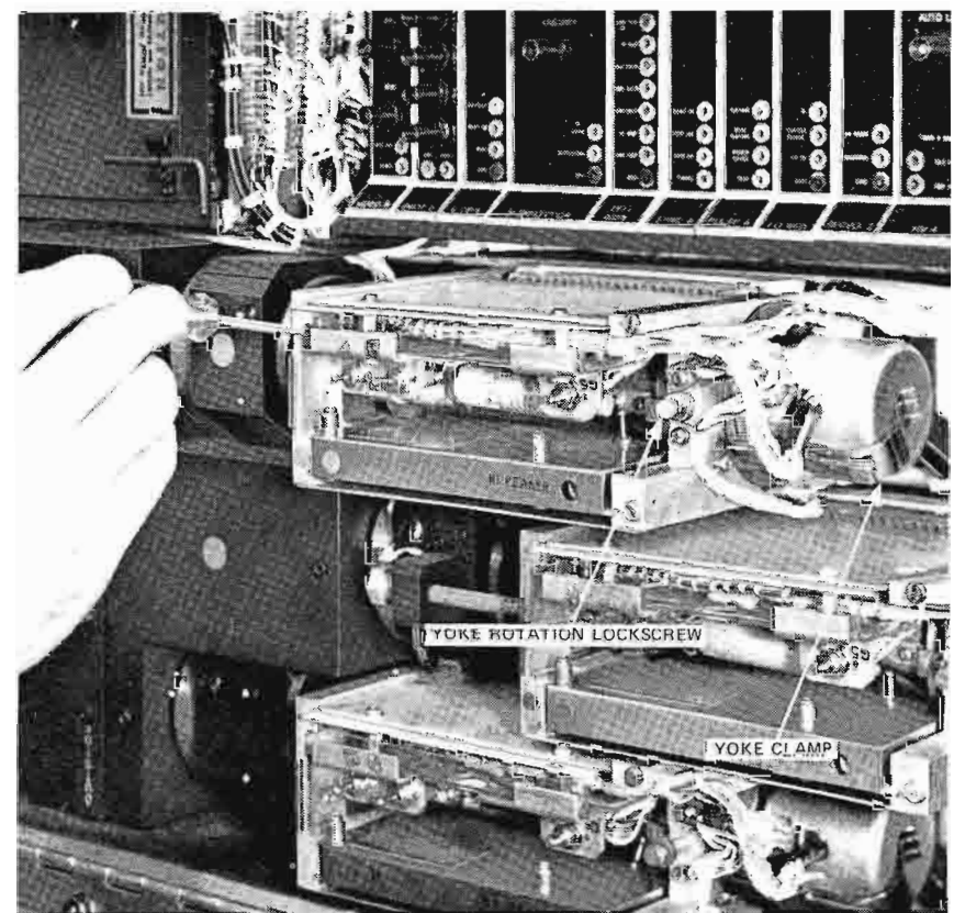
FIG. 6 Screwdriver is shown on vidicon locking screw.
