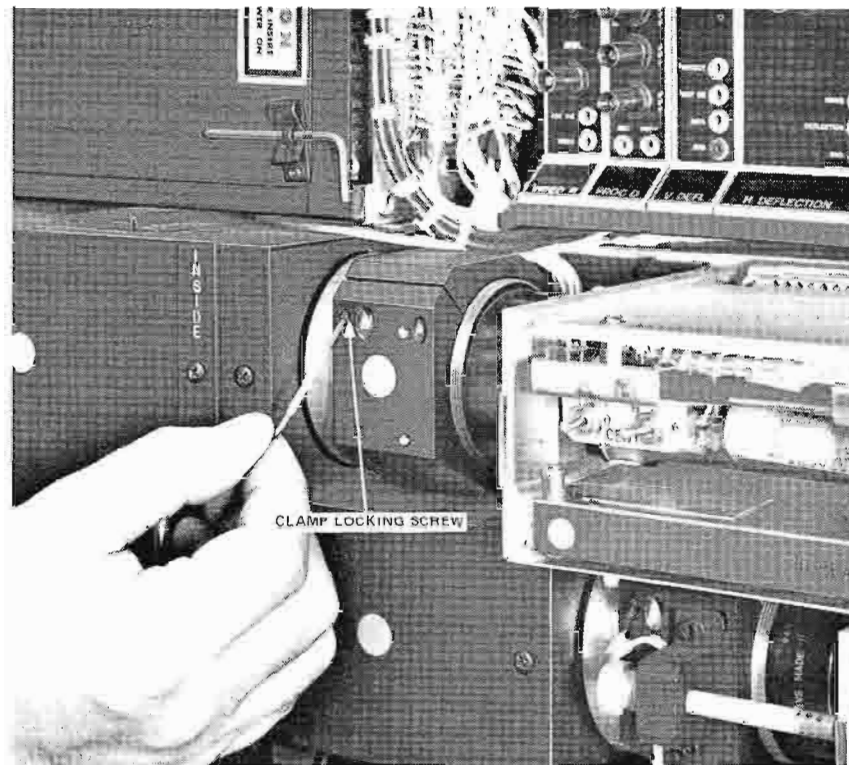
FIG. 8 Allen key shown on clamp expanding screw.
