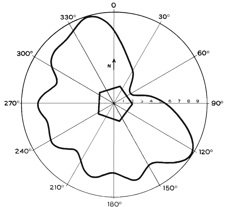
FIG. 8 Primary coverage area centered on Chicago is bisected by Lake Michigan. The horizontal radiation patterns of the UHF Polygons were tailored to meet this condition as shown.
