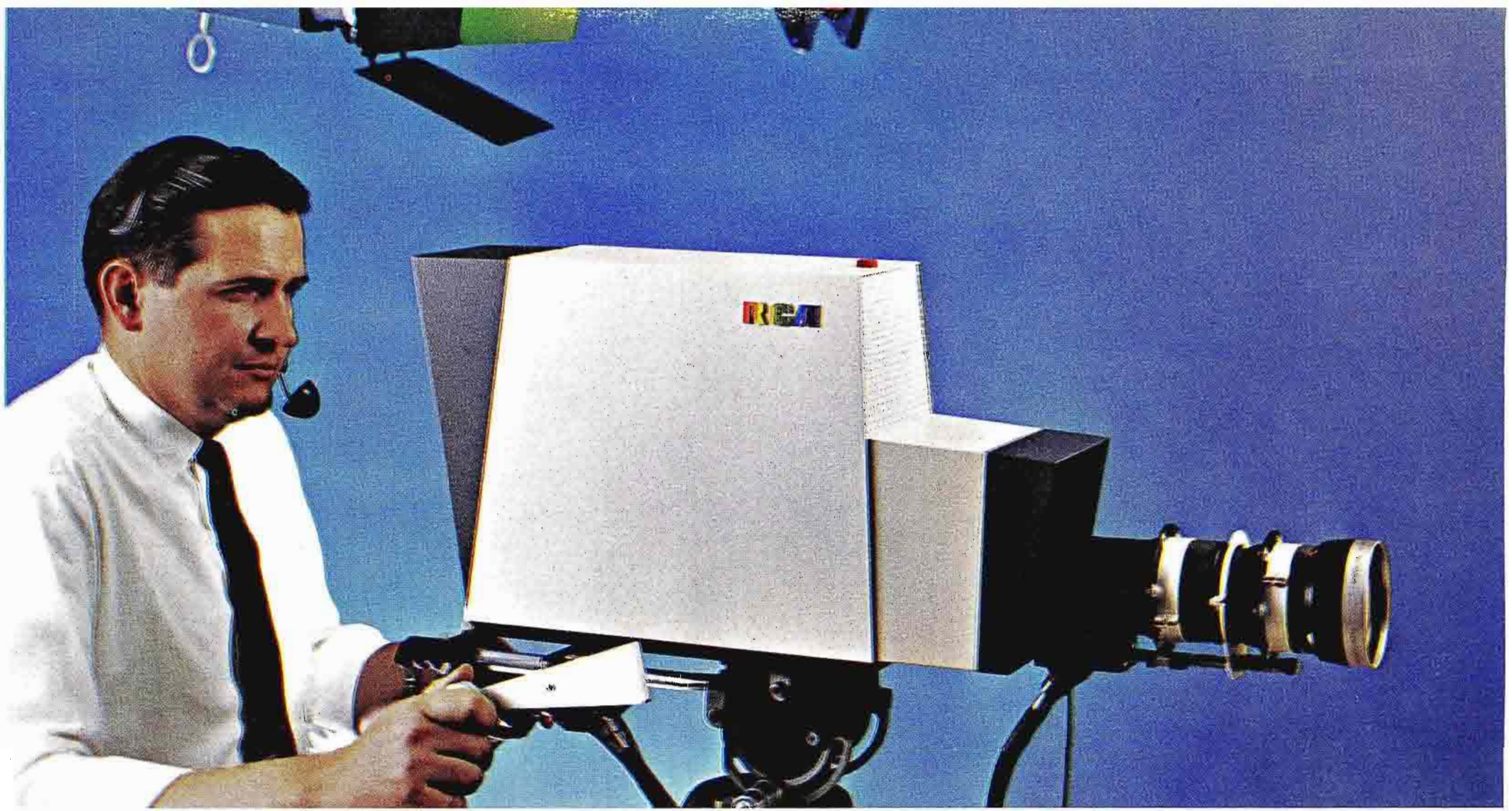
FIG. 1 New single-tube solid-state live color camera, Type PK-730. This is a viewfinder camera with 6:1 zoom lens.
