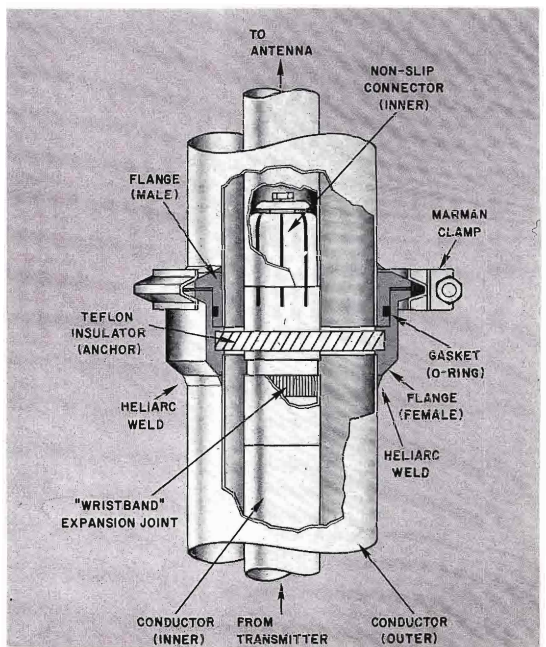
FIG. 3 Universal line coupling in cross-section. The "sexed" coupling prevents misalignment during installation and the fully-captive "O-ring" gasket assures a leakproof joint.
