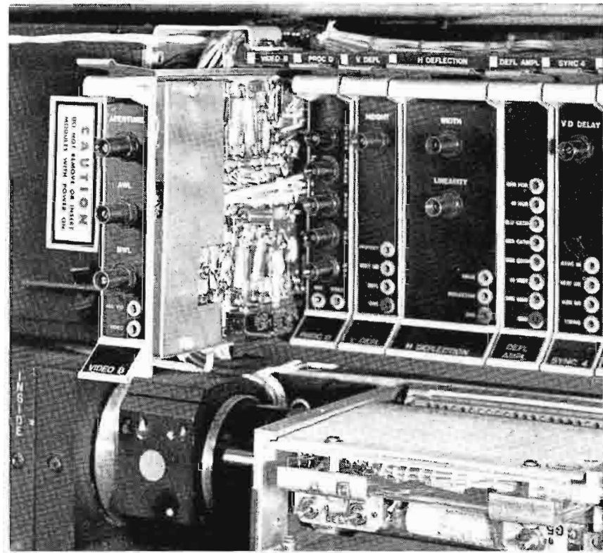
FIG. 3 Video B module for improved S/N ratio.
