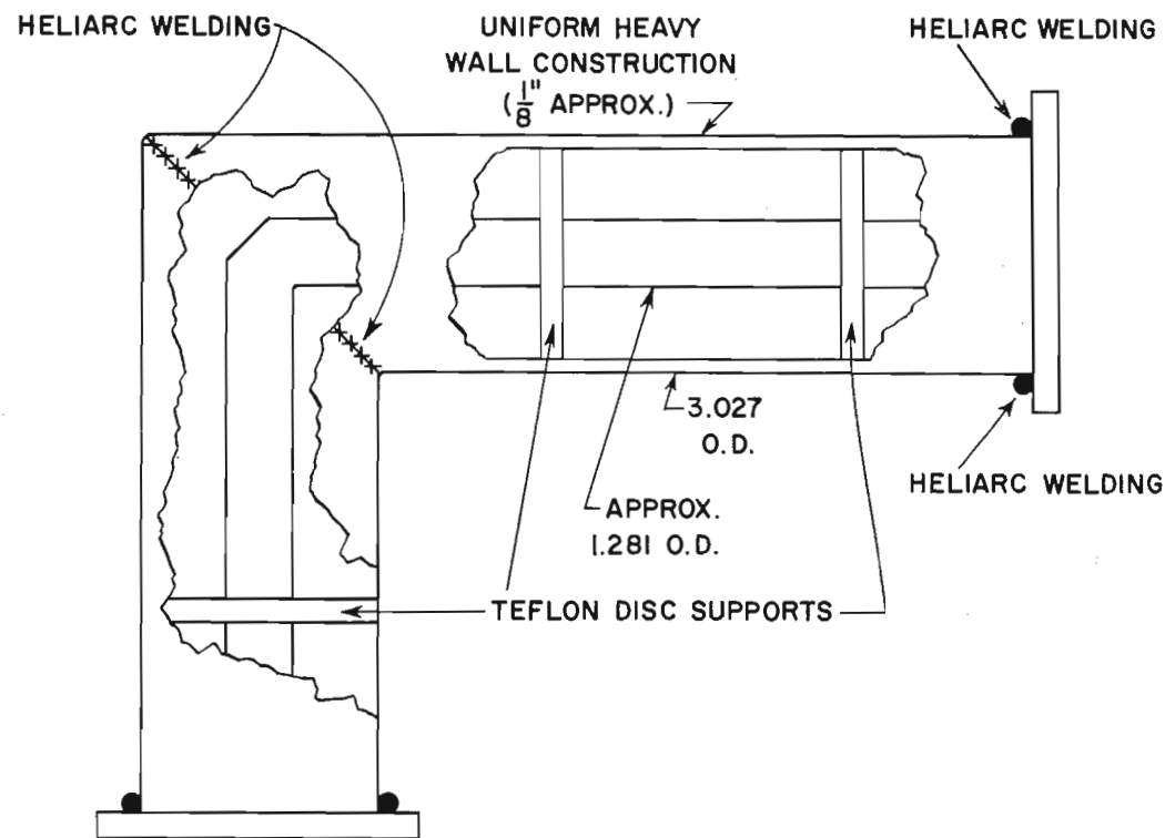
FIG. 1 Cutaway of miter elbow showing method of inner conductor support.
