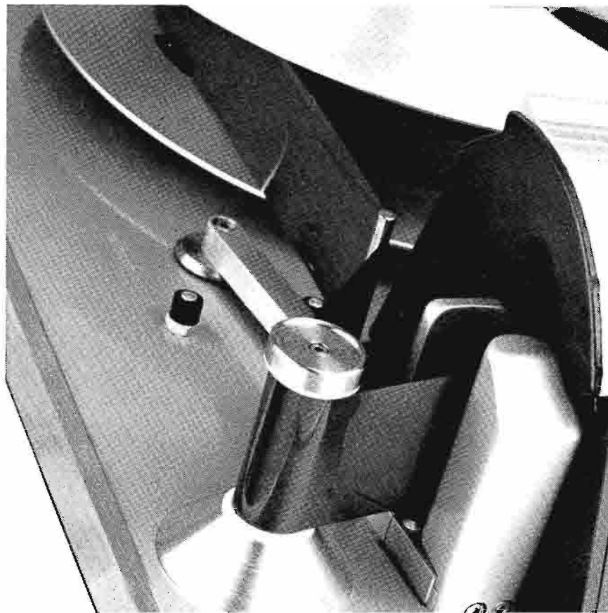
SCRATCHLESS ERASE HEAD erases from base side of the tape to eliminate any possibility of scratching the oxide.
